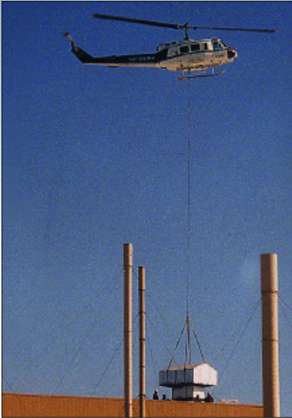
Fabrication & Installation, Intake Hood of an Air Supply House Project (above/below)
